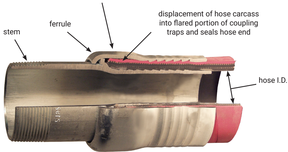
cross-section of Holedall externally swaged assembly
